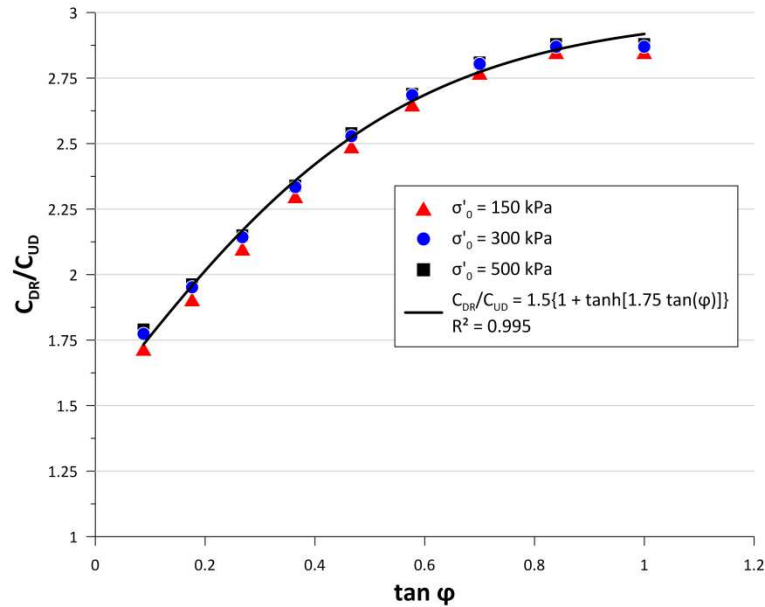
Figure 8. Drained to undrained torque ratio as a function of the friction angle.
