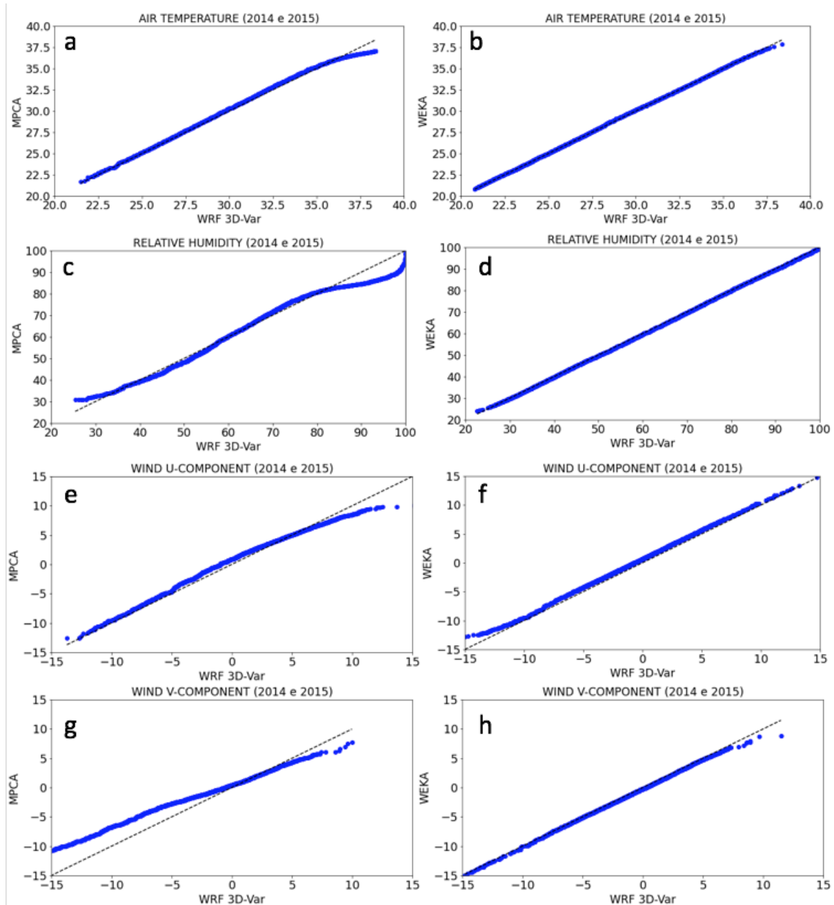
Figure 2. Quantile-quantile plot comparing the probability distribution of the trained neural networks (MPCA and Weka) (y-axis) and the actual values (x-axis) for air temperature (a and b), relative humidity (c and d), wind u -component (e and f) and wind v -component (g and h). The dashed line represents the perfect correspondence (1:1) between the trained neural network and the 3D-Var approach.
