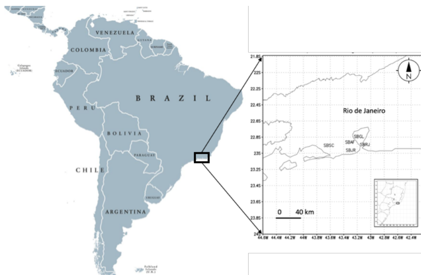
Figure 1. Study area and sensor locations. The codes in the zoom represent the ICAO identifications codes for Santos Dumont Airport (SBRJ), Galeão International Airport (SBGL), Santa Cruz Air Force Base (SBSC), Jacarepaguá Airport and Afonsos Air Force Base (SBAF).
