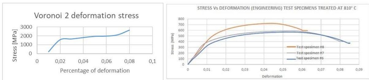
Figure 9. Stress vs. strain diagrams for artificial models and comparison of results
